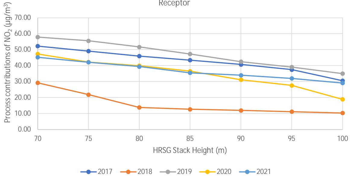
99.79 th Percentile of the Hourly NO 2 Process Contributions at the Most Affected Receptor
