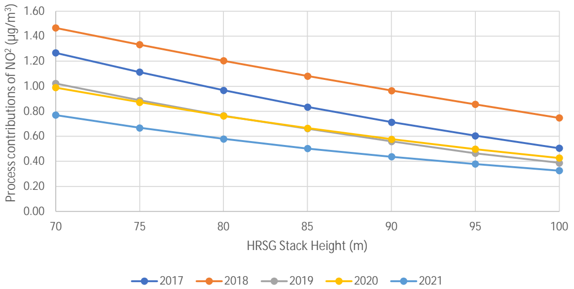
Annual Mean NO 2 Process Contributions at the Most Affected Receptor
