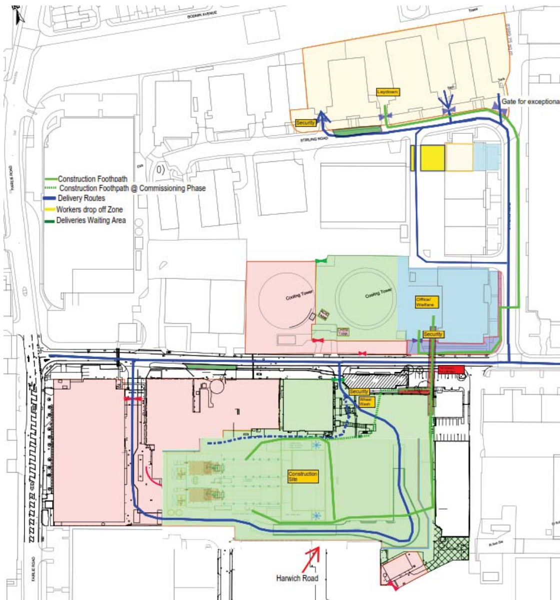
Figure 3: Site Layout
